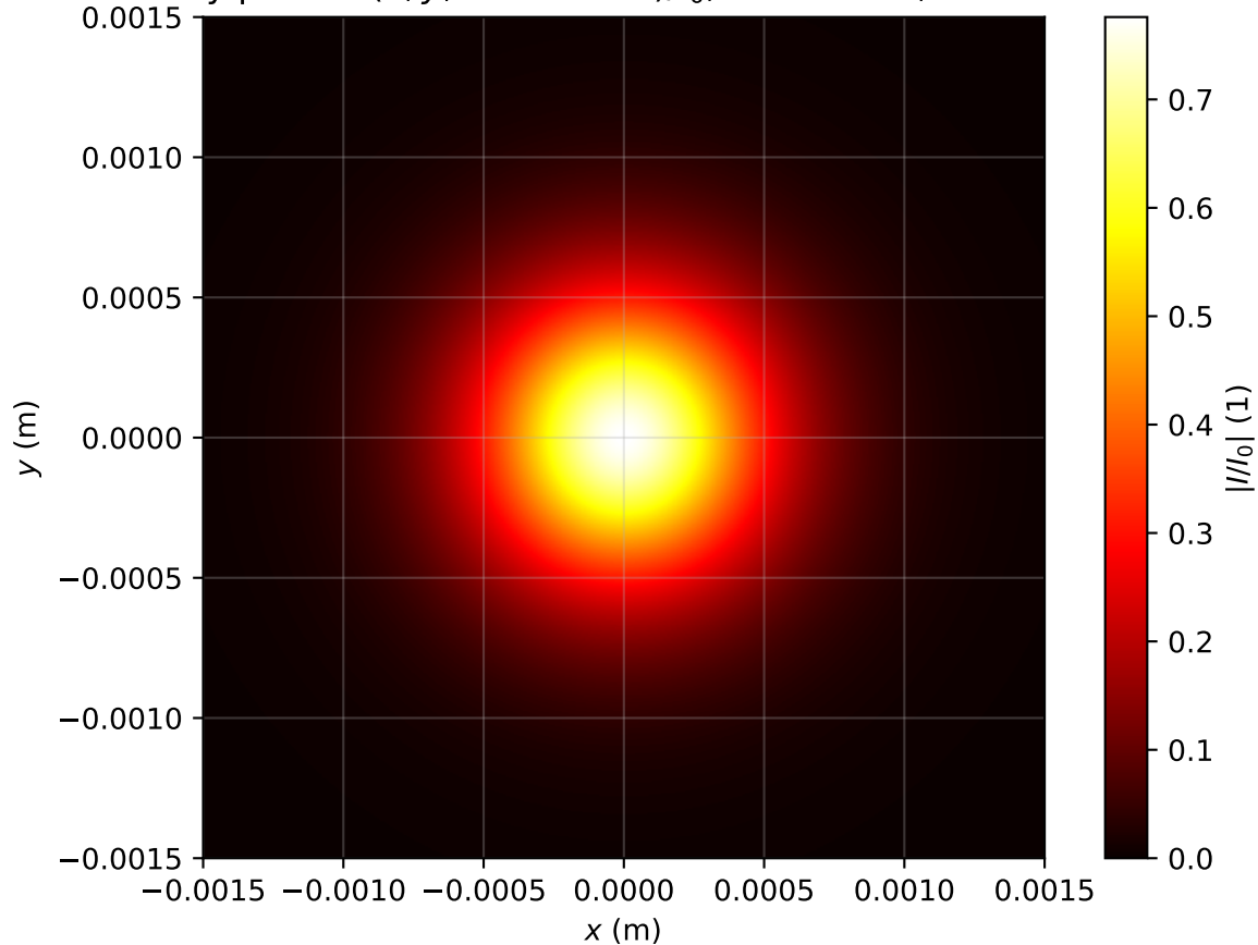
Intensity profile I(x, y, z = 3.264m)/I_0 , Pin=0.7Pcr, artificial time
